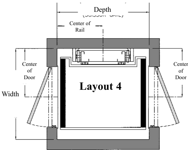
Opposite Opening Car Right Hand Door/Left Hand Door
