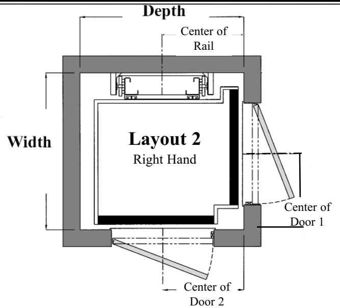
90 Deg. Car Right Hand Door/Left Hand Door
